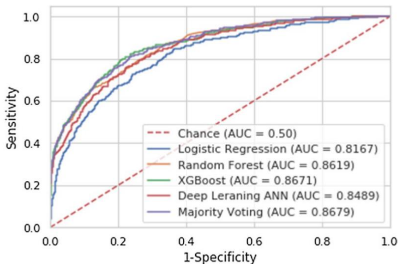
Figure 13: AUC of several machine learning models
