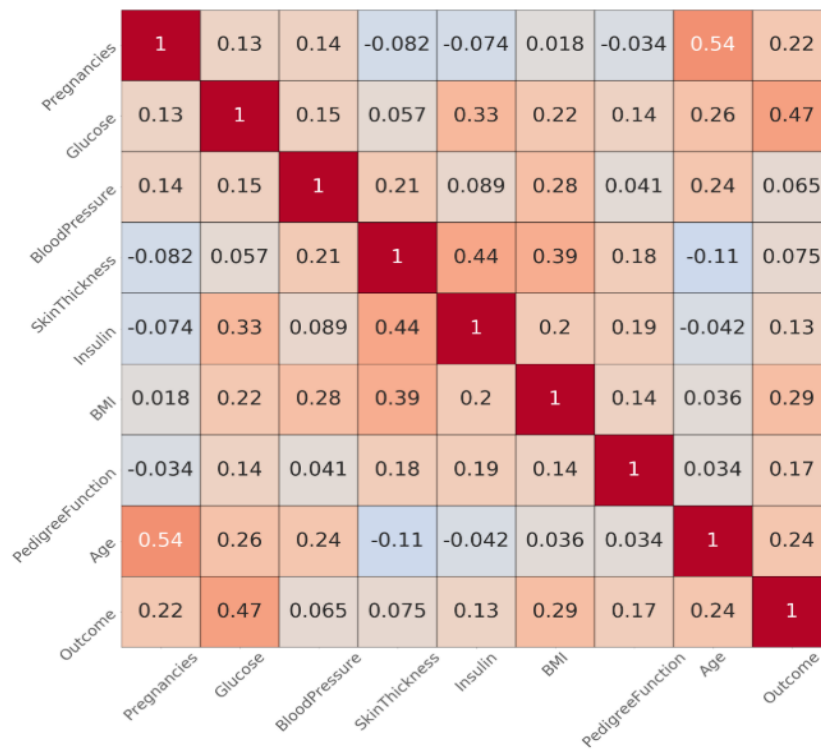
Figure 14: Dataset correlation matrix
