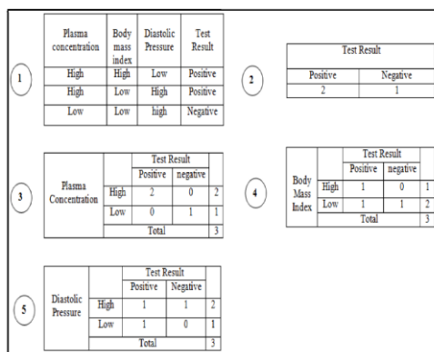
Figure 11. Decision tree in action for diabetic prognosis
